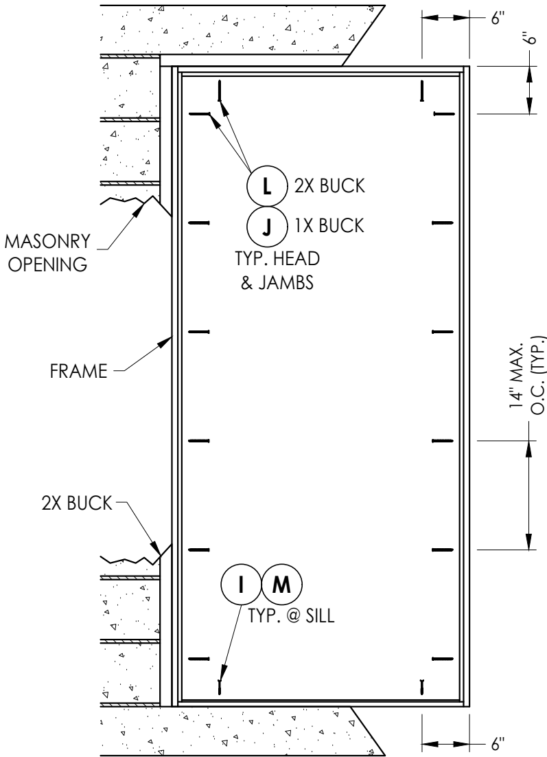
FRAME ANCHORING
