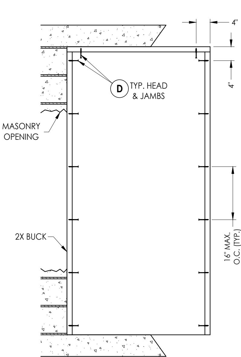
BUCK ANCHORING
