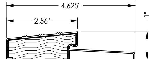
31 OUTSWING THRESHOLD
